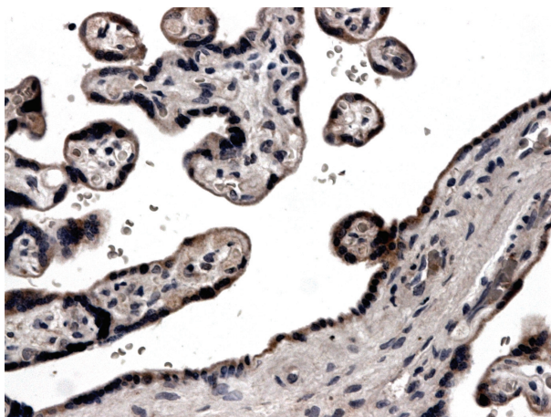
Formalin fixed and paraffin embedded normal human placenta tissue is subjected to mouse anti human TIMP-4 (hAP-0037)
